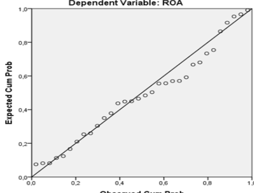
Normal P-P Plot of Regression Standardized Residual Dependent Variable: ROA
